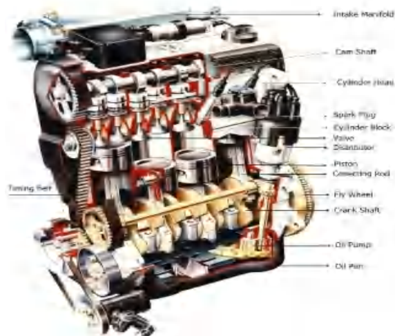
Gambar 2. Mesin diesel
