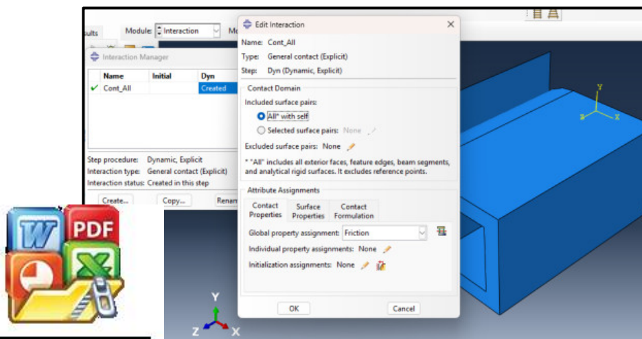
Gambar 23. Tampilan Interaction
