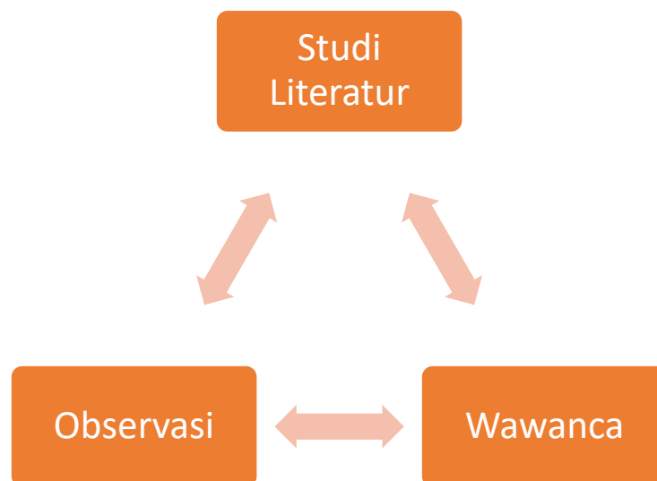
Gambar 2. 1. Triangulasi Data
