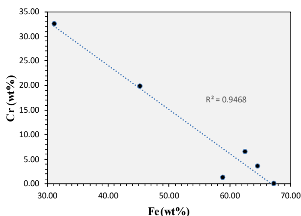
Fig. 6 Binary diagram showing the strongly negative correlation between Cr and Fe of the iron-rich minerals.
