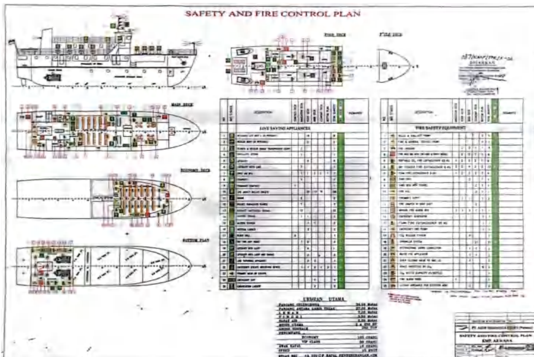
Lampiran 6 Gambar general arrangement KMP. Arwana
