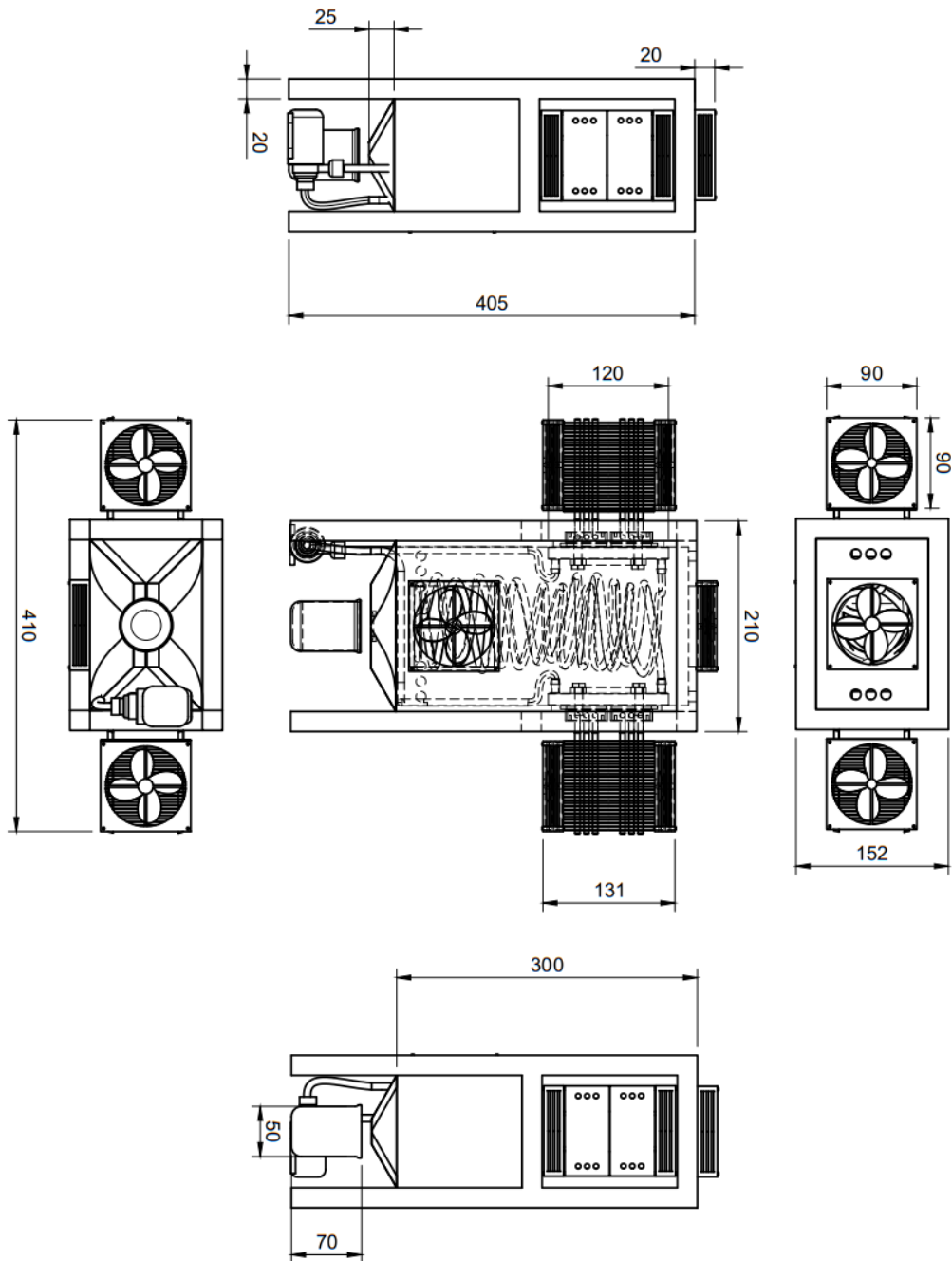
Lampiran 1 Dimensi Atmospheric Water Generator
