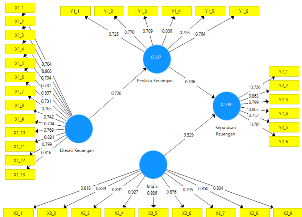
Gambar 7.1 Model PLS
