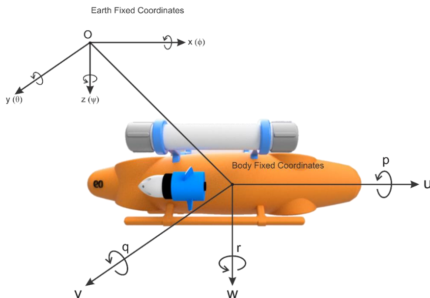
Gambar 7. Sistem koordinat fixed-fix dan earth-fixed.
