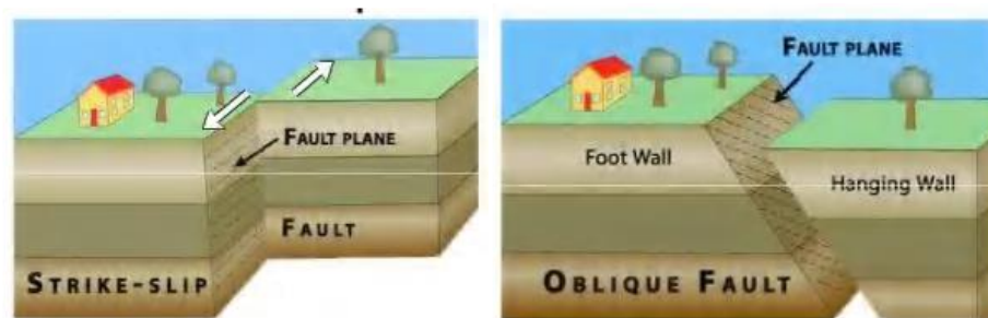
Gambar 2.7 Sesar mendatar ( Strike – slip fault ) dan Sesar Oblique ( Oblique fault ) (Ibrahim dkk., 2010)
