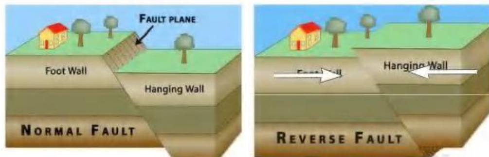
Gambar 2.8 Sesar turun ( Normal fault ) dan sesar naik ( Reverse fault ) (Ibrahim dkk., 2010)
