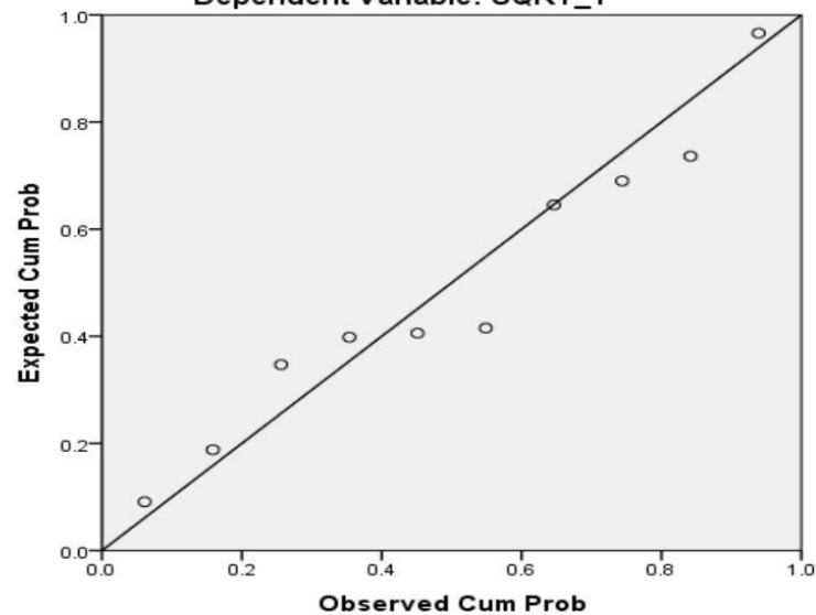
Normal P-P Plot of Regression Standardized Residual Dependent Variable: SQRT_Y
