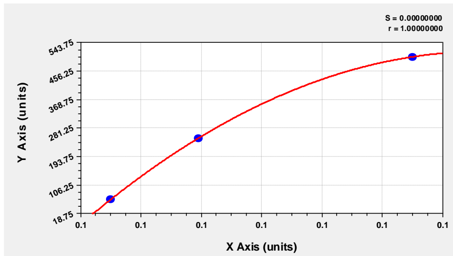
Kurva standar BSA
