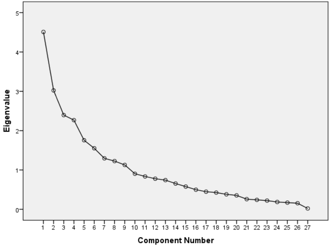
Scree Plot
