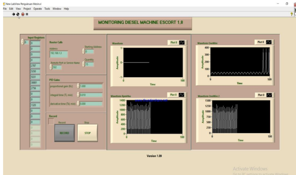
Gambar Human Machine Interface saat merekam
