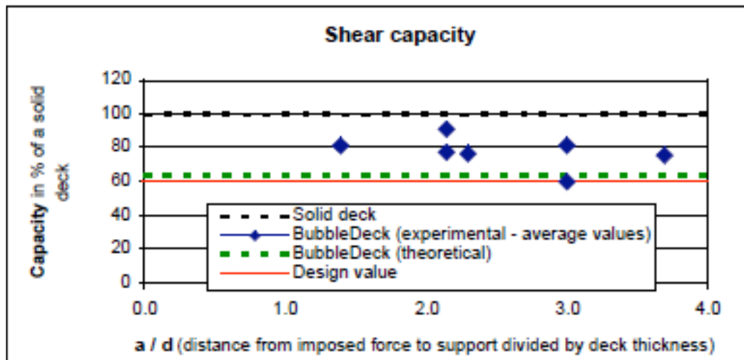
Gambar 13. Grafik Kapasitas Geser Pelat Beton Bertulang Berongga Bola (“Bubble Deck Tesis and report Summary” Issue 1 June 2006 )
