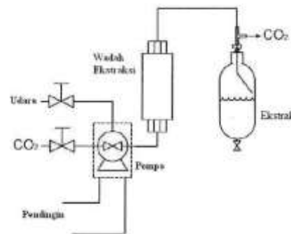
Gambar 8. Rangkaian Alat Supercritical Fluid Extraction (Juliando, 2019)
